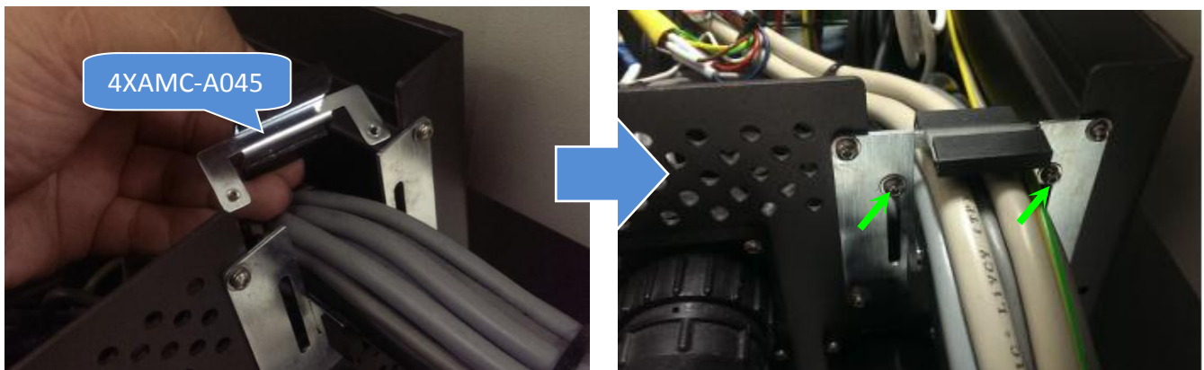
Figure 52 Holding Plate Assembly
