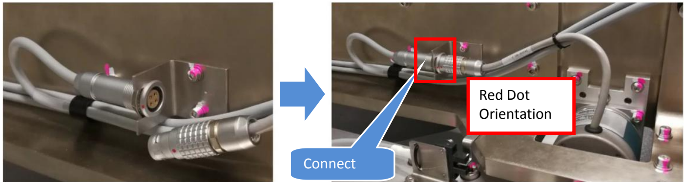
Figure 33 Stepper Motor Cable Connect
