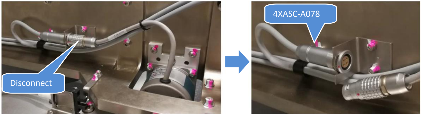
Figure 3 Left Stepper Motor Connector Removal
