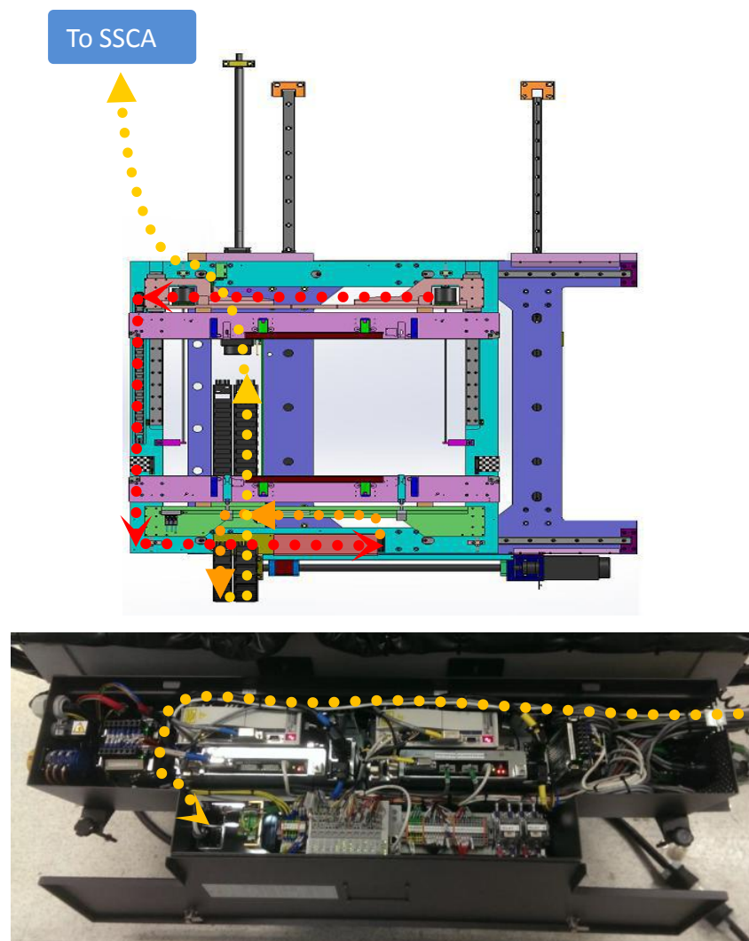
Figure 4 Left Stepper Motor Cable Routing
