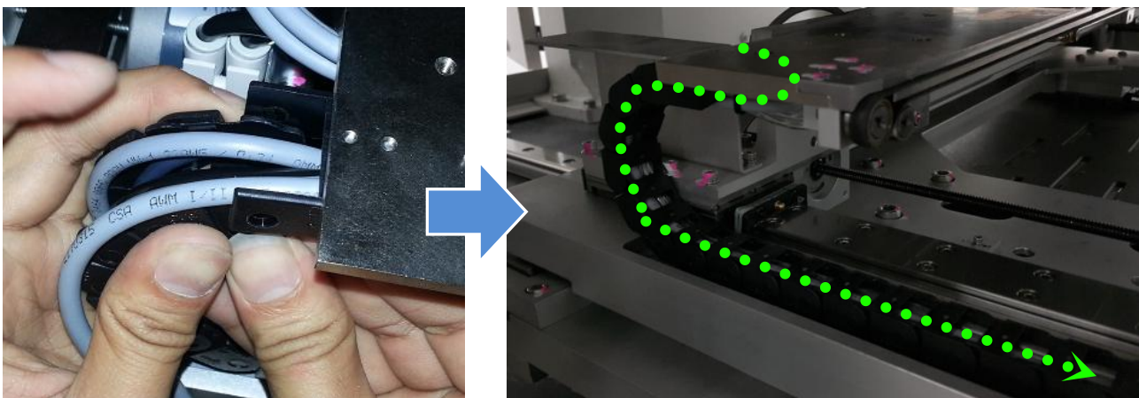
Figure 34 Stepper Motor Cable Routing (AWA E-Chain)
