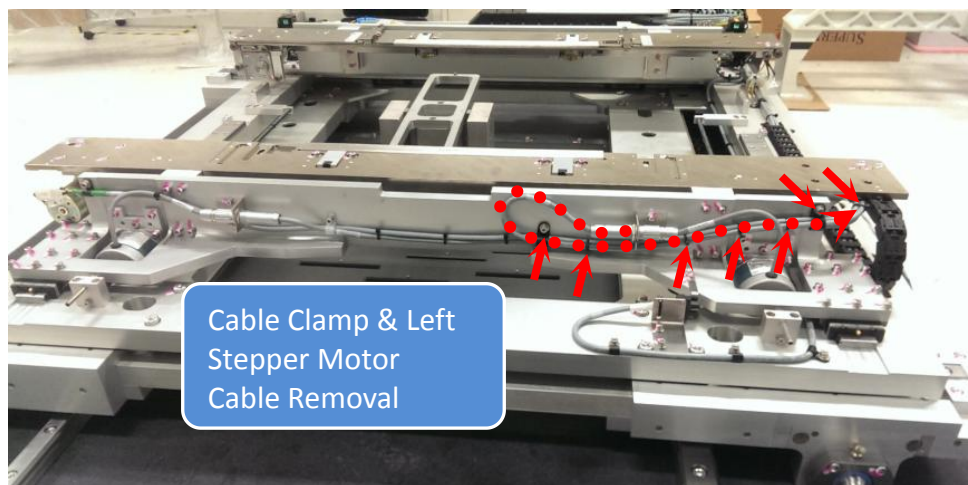
Figure 6 Cable Clamp & Left Stepper Motor Cable Removal
