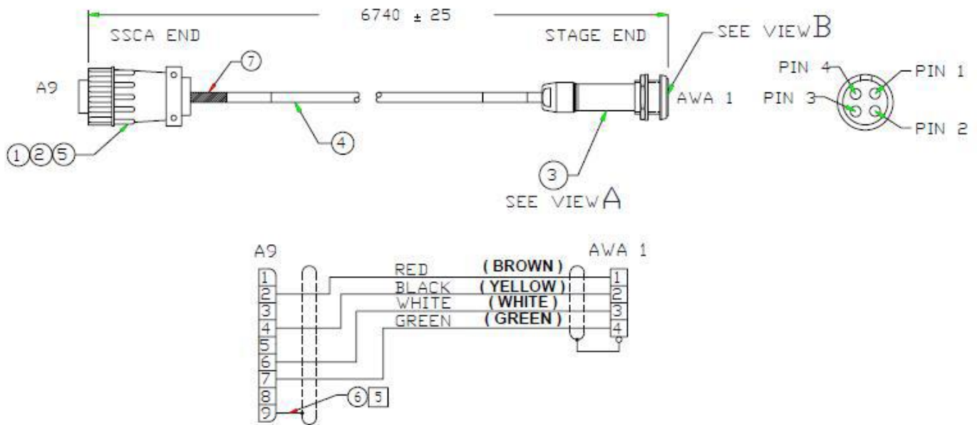
Figure 29 Cable Drawing
